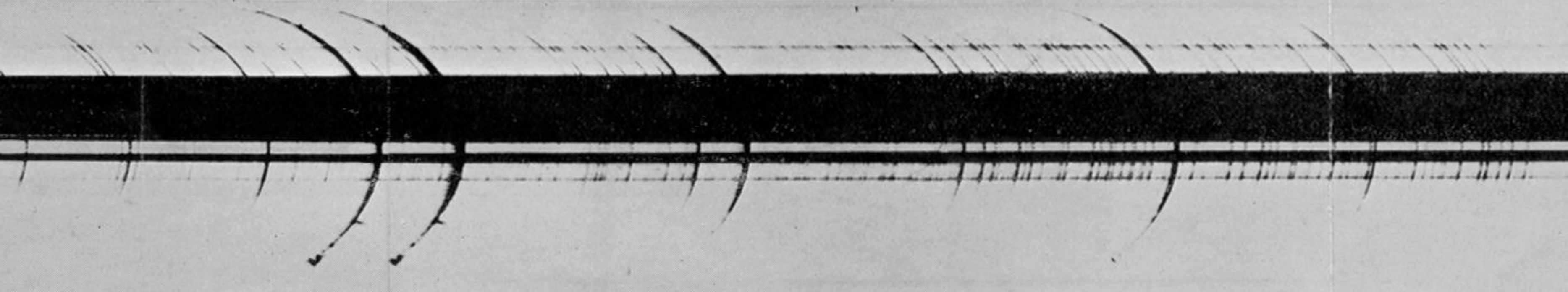
10. Exposed for 2 seconds, beginning 10 seconds before mid-eclipse.
