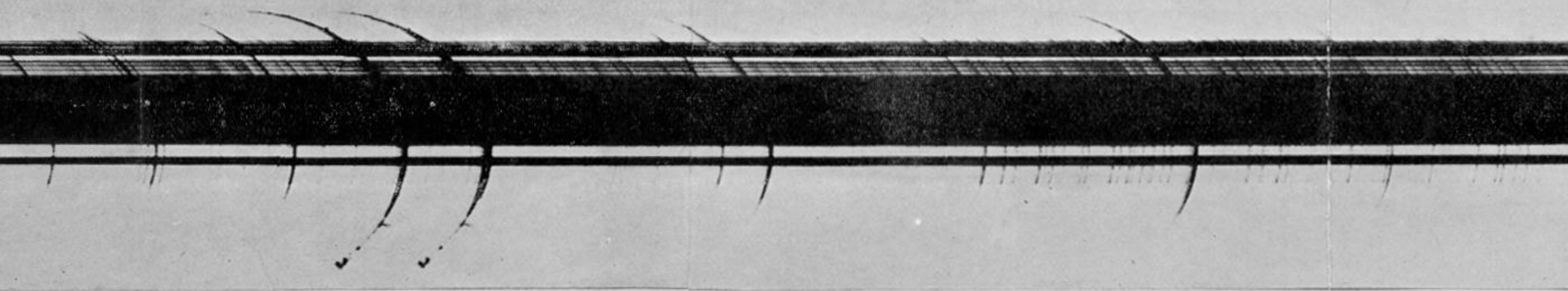
9. Exposed for 2 seconds, beginning 15 seconds before mid-eclipse.
