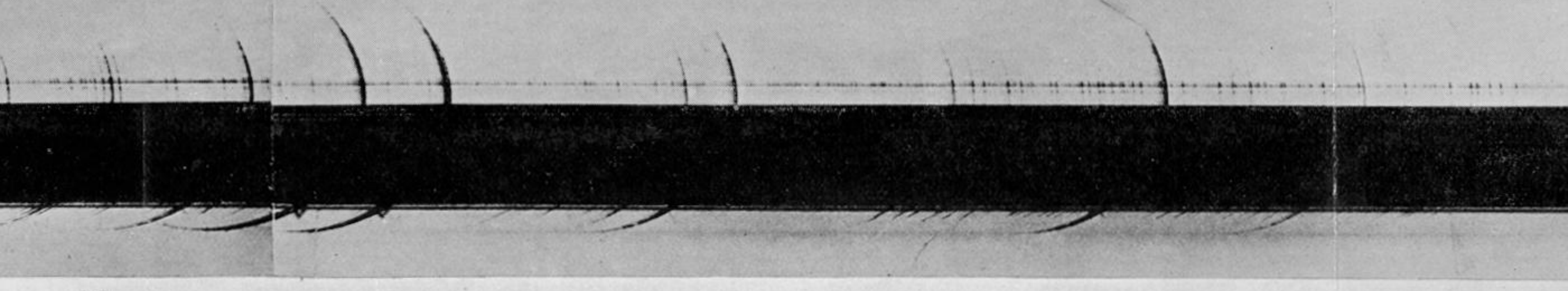
13. Exposed for 2 seconds, beginning 14 seconds after mid-eclipse.
