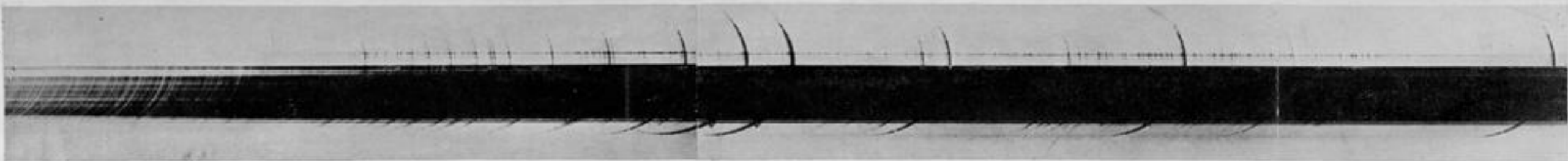
SPECTRUM N° 13. Exposed for 2 seconds, beginning 14 seconds after mid-eclipse.
